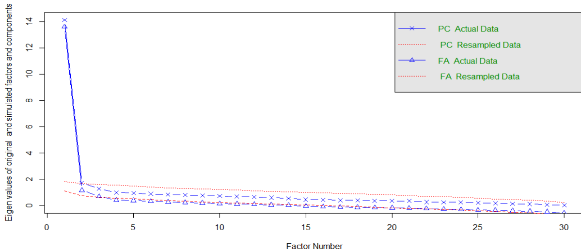
Figure 1: Eigenvalues of tetrachoric matrix
